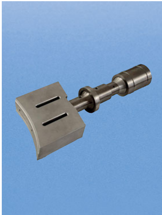
Sonotrode for integration into standard and special systems
