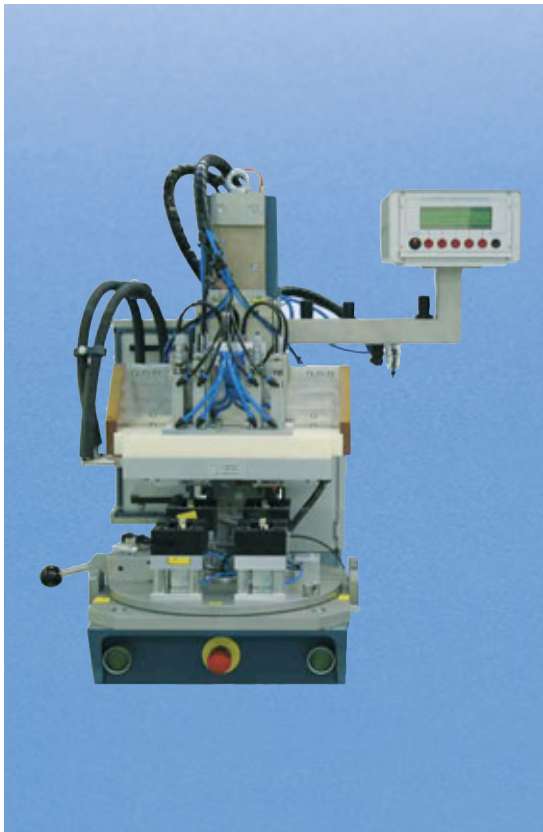
ERW thermal installation machine to embed eight inserts M 1.6 into two mobile phone half shells
